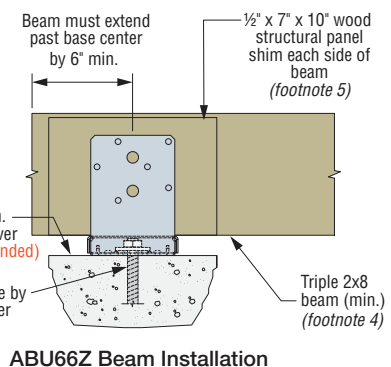
ABU66Z Beam Installation
