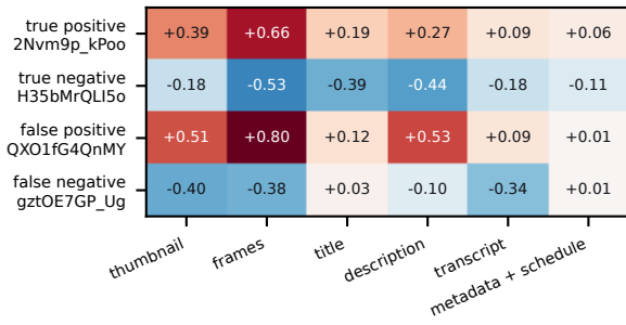
(b) Exact logit contributions for seed-0 examples
