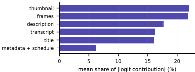
(b) Exact logit contributions for seed-0 examples
