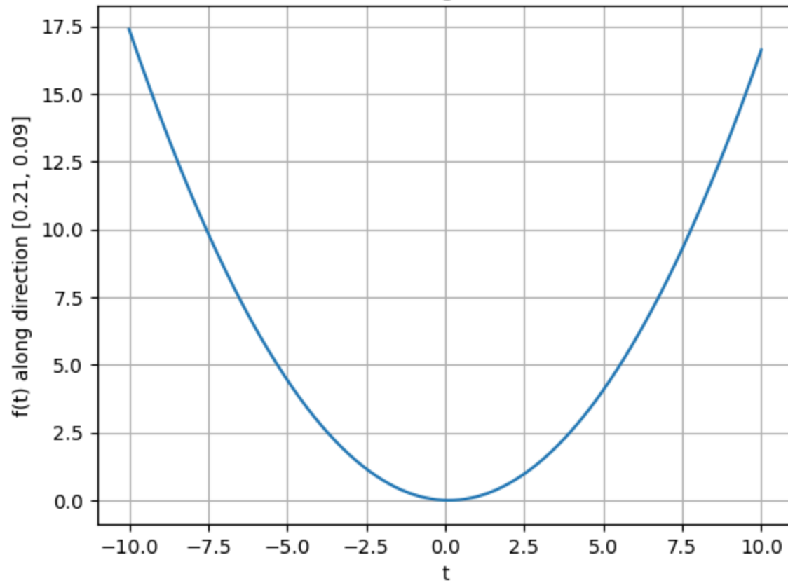
Function f(x_1, x_2) along Direction [0.21, 0.09]
