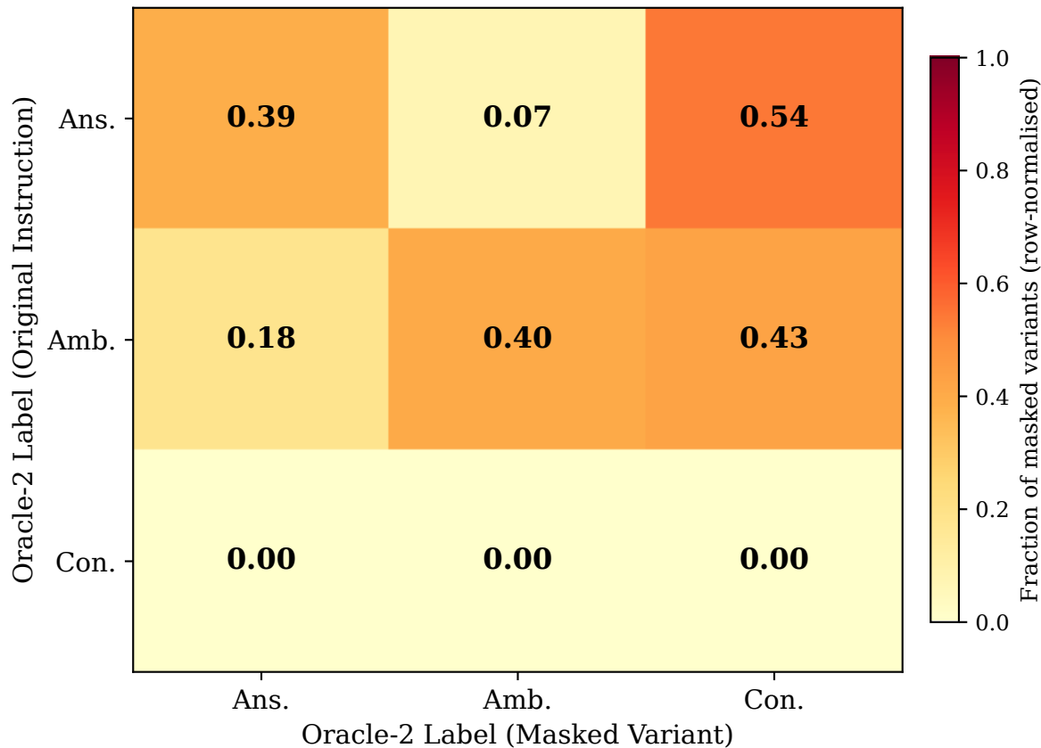
Original vs. Masked Variant Oracle-2 Label Transition (Row-Normalised) How masking reshapes the label distribution
