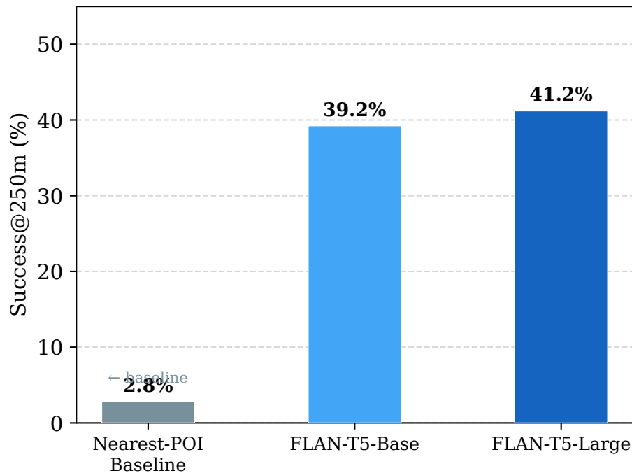
Goal Localization Accuracy (Resolved Predictions Only)
