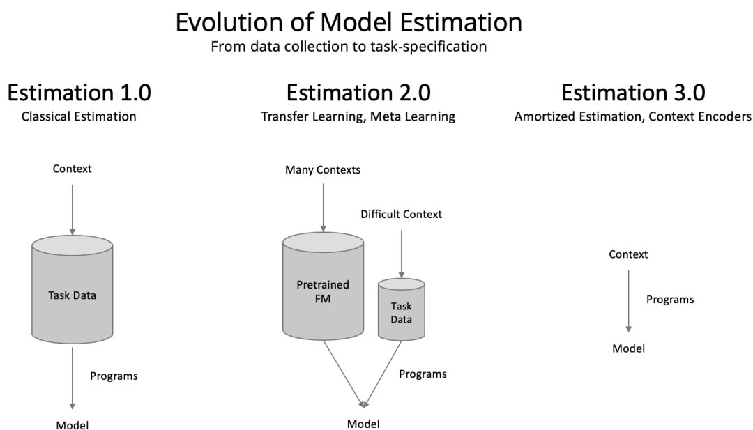
Figure 10: Evolution of Statistical Estimation. Classical estimators (left) require sufficiently large context-specific datasets for single-instance learning. Meta-learning and transfer learning (middle) decrease the need for context-specific data collection, but still perform a few rounds of gradient descent on context-specific data. Finally, amortized estimators (right) only use a representation of the data context to produce new model parameters, handling data collection and classical estimation implicitly.
