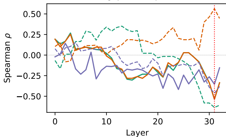
Steering (peak L31, \rho=-0.636 )
