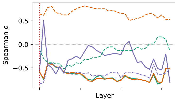
Steering (peak L31, \rho=-0.636 )
