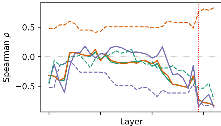
MIA (peak L01, \rho=0.549 )
