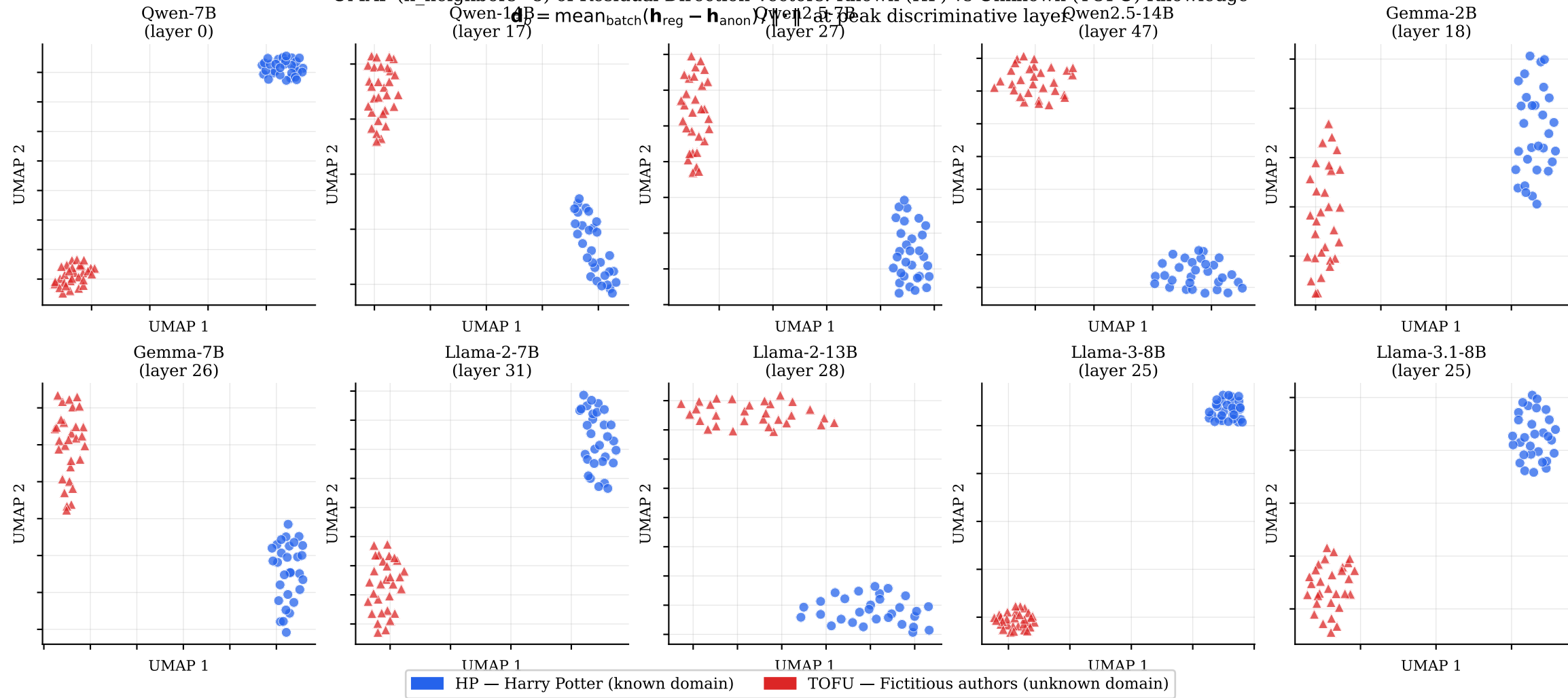
UMAP (n_neighbors=8) of Residual Direction Vectors: Known (HP) vs Unknown (TOFU) Knowledge
