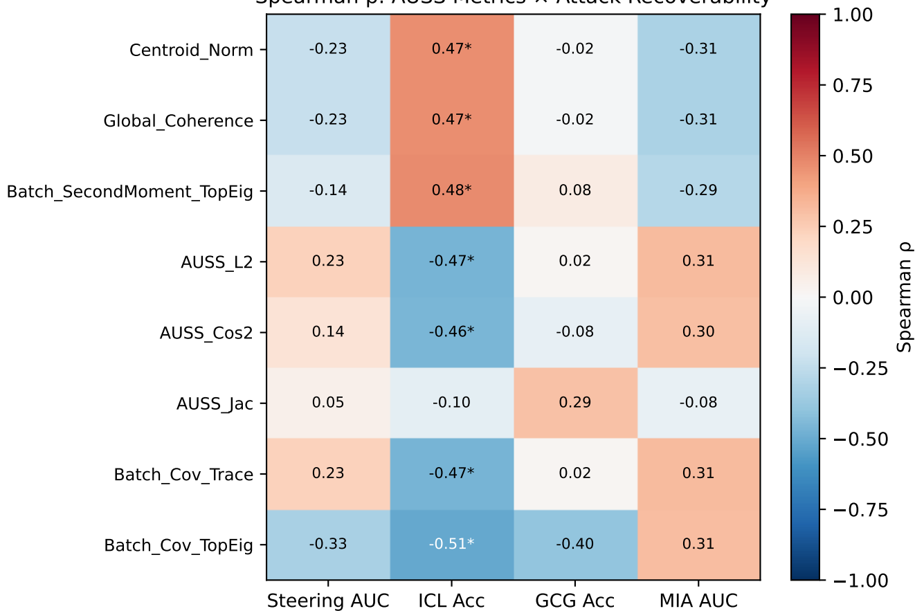
Spearman \rho : AUSS Metrics \times Attack Recoverability
