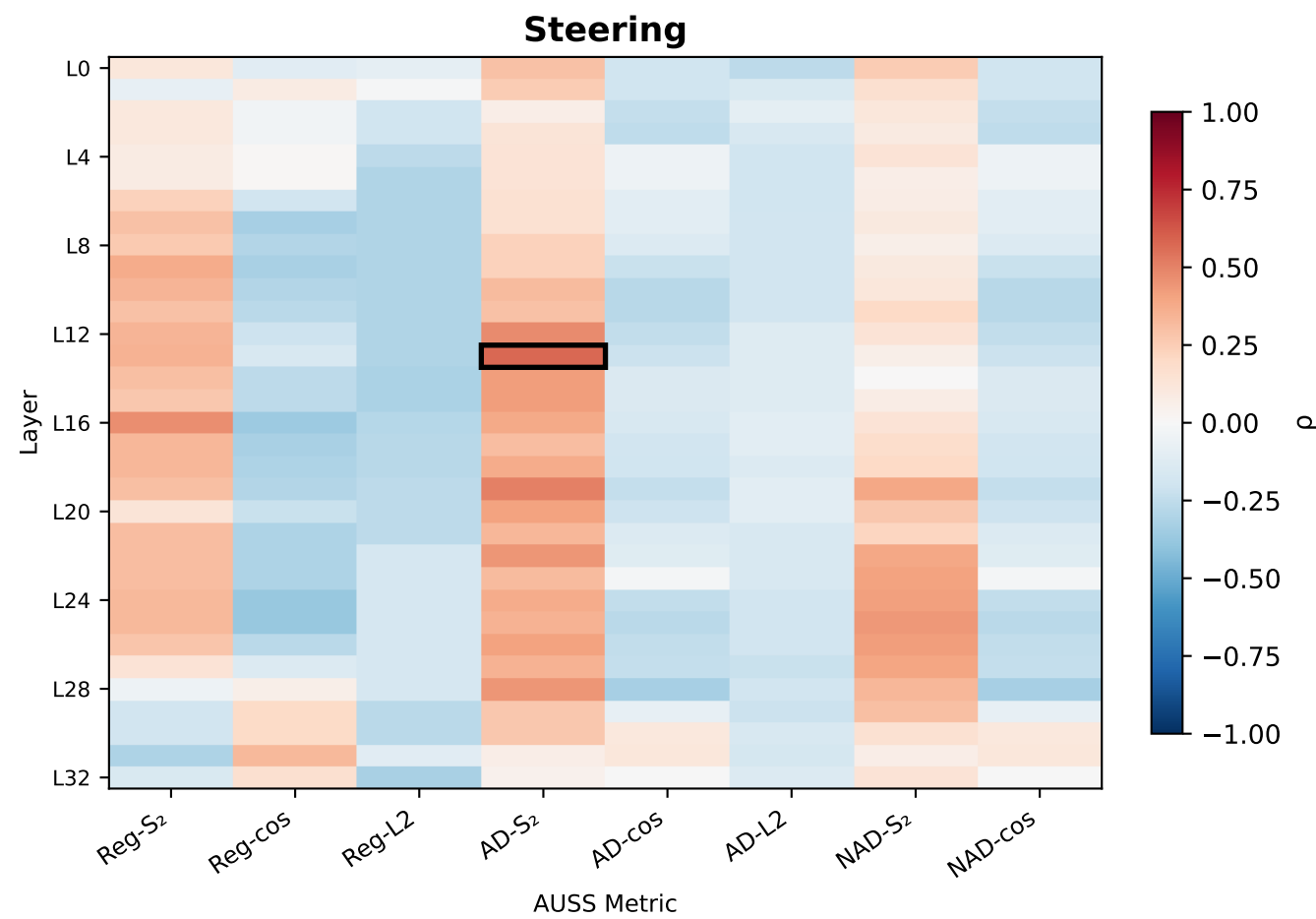
Per-Layer AUSS × ASR Spearman \rho (black box = |\rho|_{\max} )
