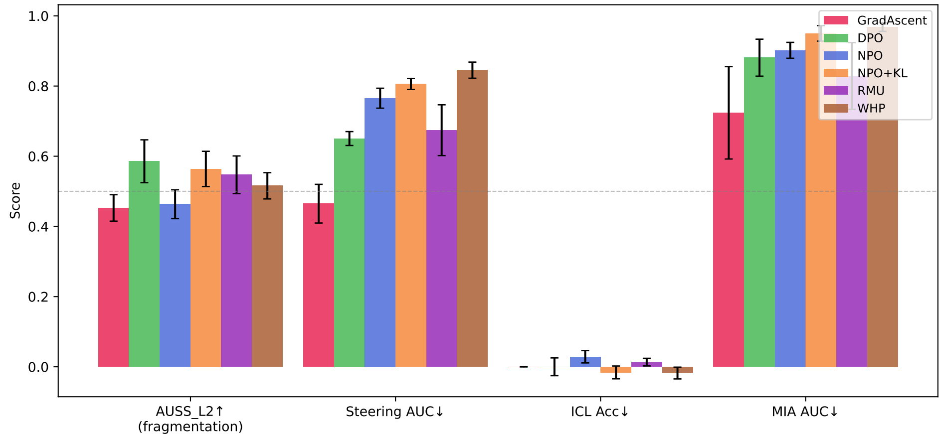
Unlearning Method Comparison: Fragmentation vs. Recoverability
