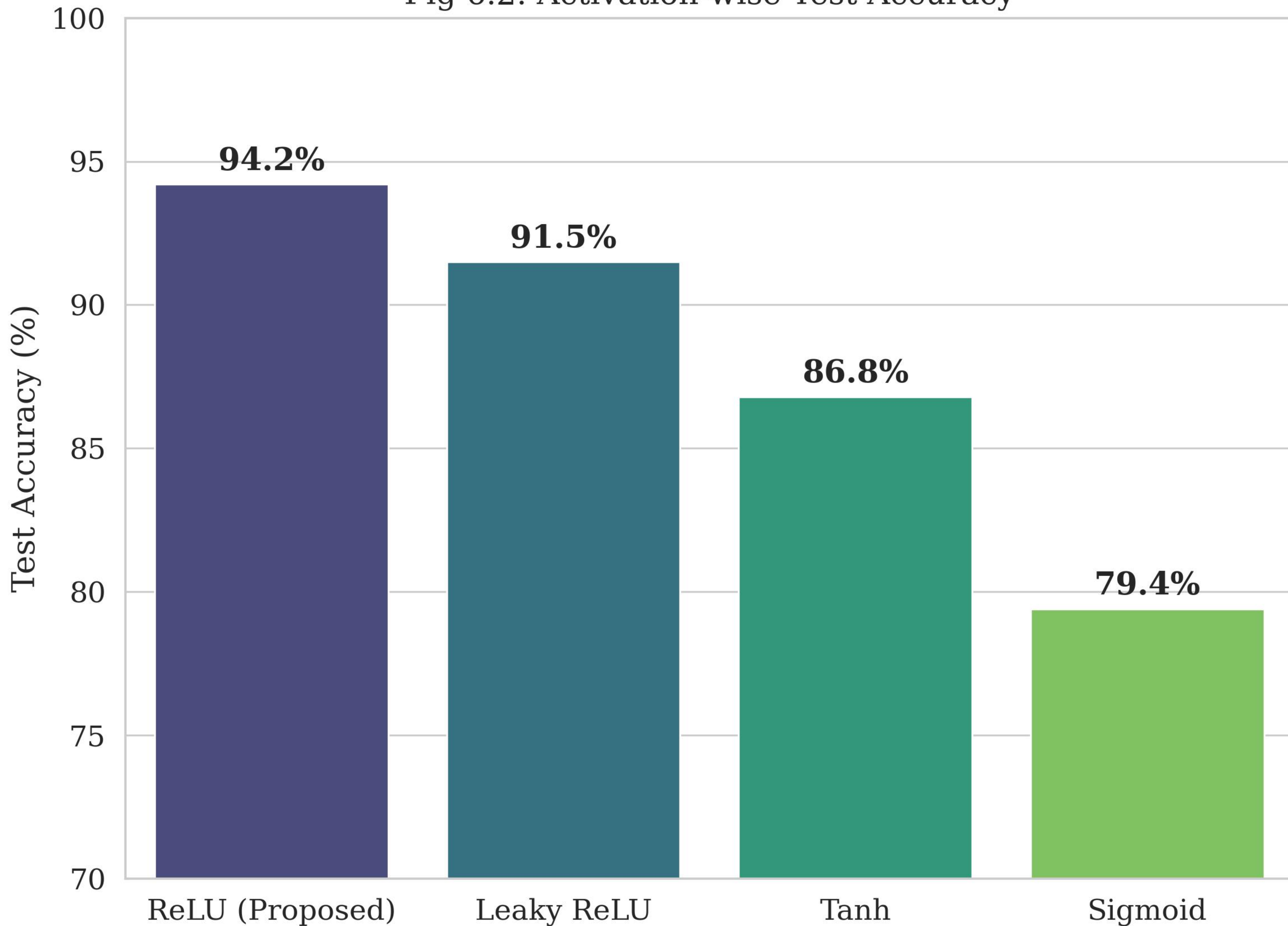
Fig 6.2: Activation-wise Test Accuracy
