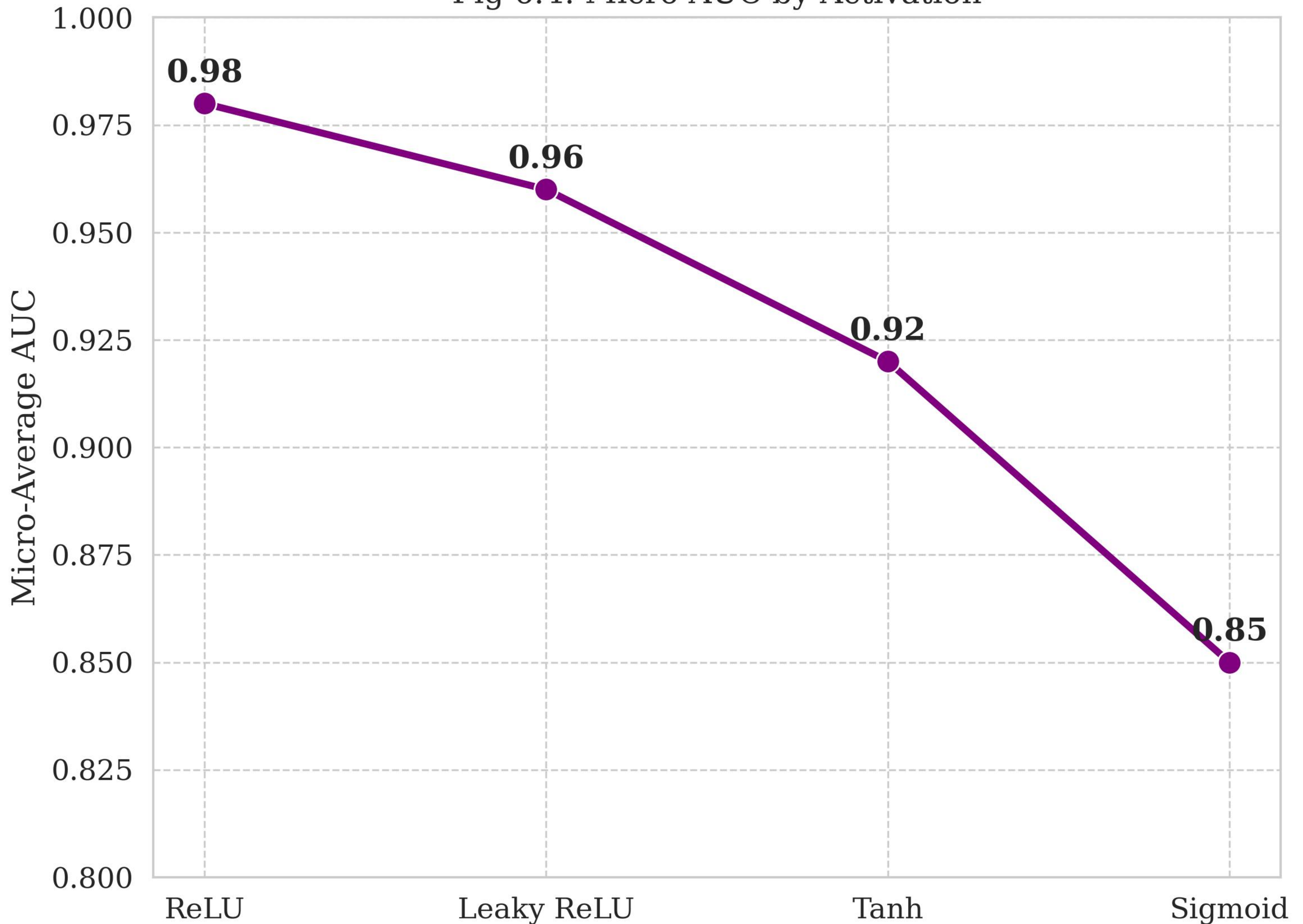
Fig 6.4: Micro AUC by Activation
