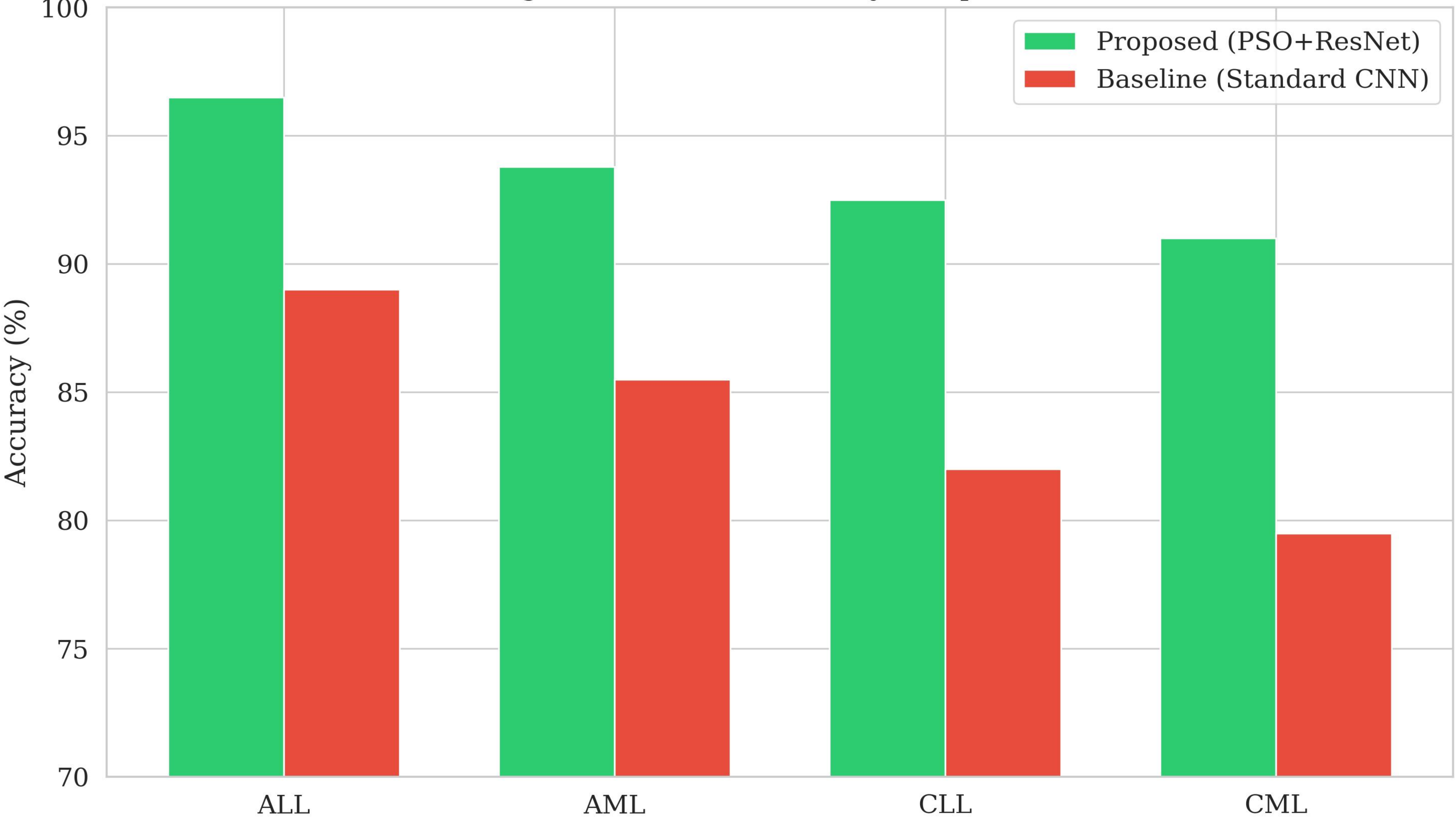
Fig 6.5: Per-Class Accuracy Comparison
