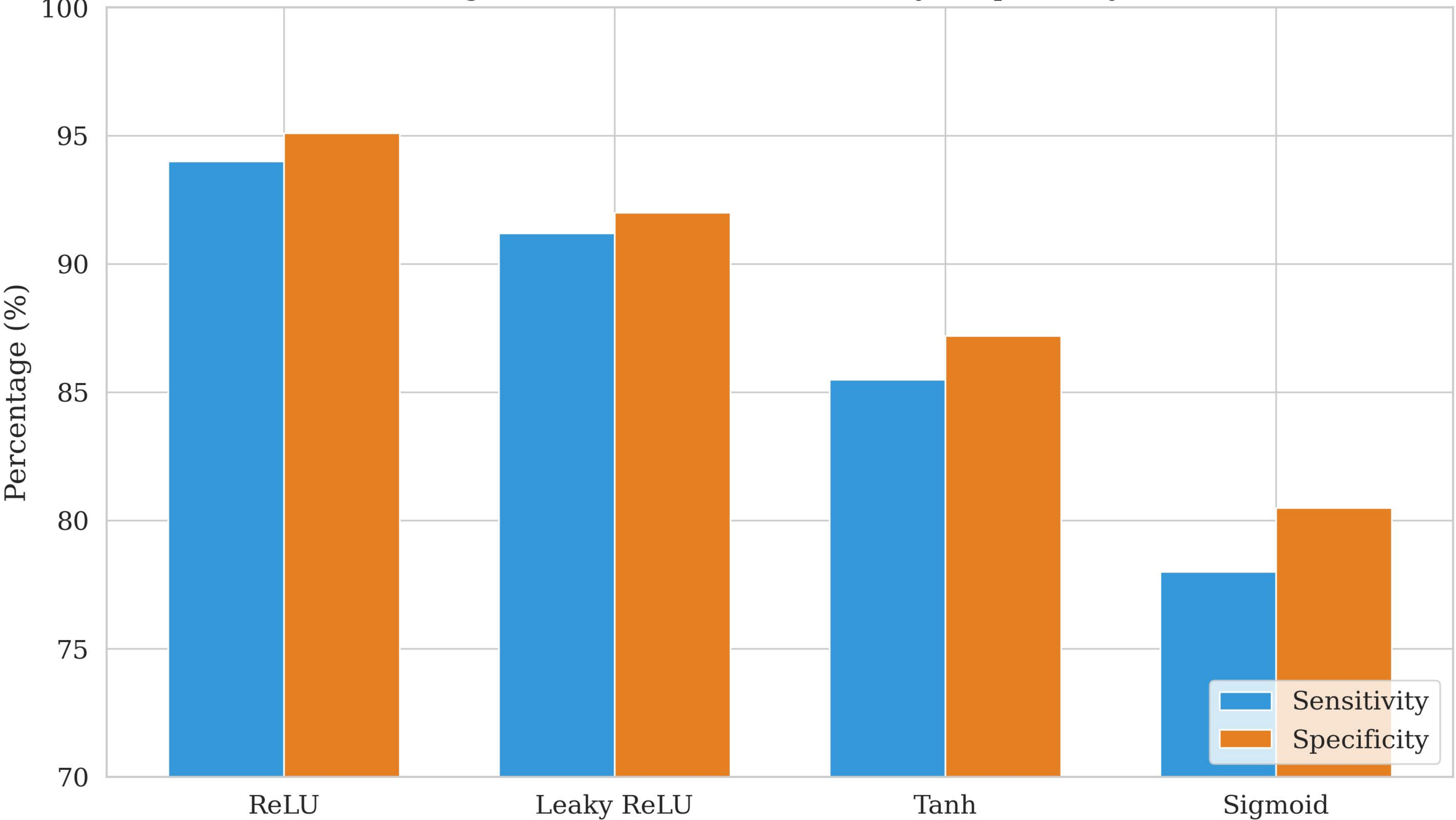
Fig 6.3: Activation-wise Sensitivity & Specificity
