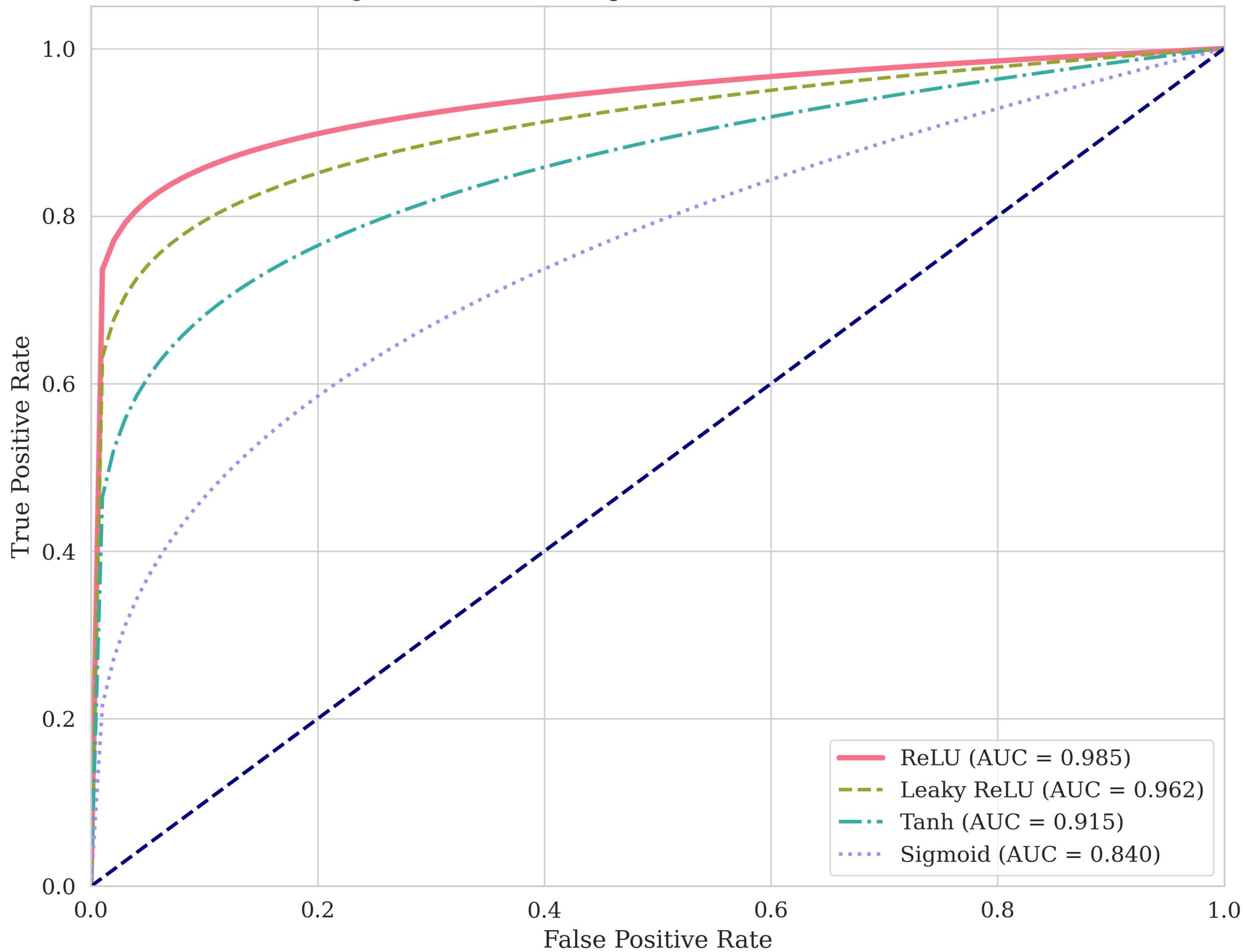
Fig 6.1: ROC-AUC Comparison of Activation Functions
