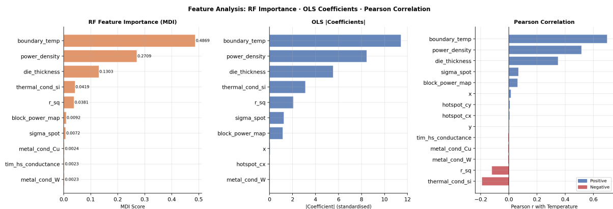
Figure 6: Three complementary ways to rank feature importance. Left: Random Forest MDI (mean decrease in impurity — how much each feature reduces prediction error in the trees). Centre: OLS absolute standardised coefficients (how strongly each feature influences the linear prediction). Right: Pearson correlations with temperature. Remarkably, all three methods agree on the top 4 features: boundary_temp , power_density , die_thickness , thermal_cond_si . The feature r_sq consistently ranks 5th in RF and OLS, confirming that spatial proximity information is actively utilised.
