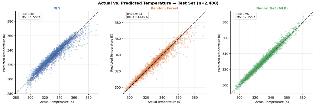
Figure 3: Scatter plot of actual vs. predicted temperature for all three model classes on the 2,400-sample test set. A perfect model would have all points on the dashed 1:1 line. The MLP plot is nearly indistinguishable from perfect prediction at this scale, with points tightly clustered around the ideal line. The OLS scatter shows more spread, especially at high temperatures (near hotspot centres) where the nonlinear Gaussian term is largest.
