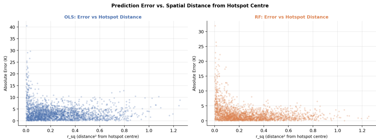
Figure 11: Absolute prediction error vs. r\_sq (squared distance from hotspot centre) for OLS and RF. With the full 14-feature dataset including spatial features, neither model shows a strong systematic pattern of high error at small r^2 . This confirms that the hotspot proximity information is now properly utilised. Without the spatial features, OLS would show dramatically increasing errors as r^2 \rightarrow 0 (near the hotspot centre).
