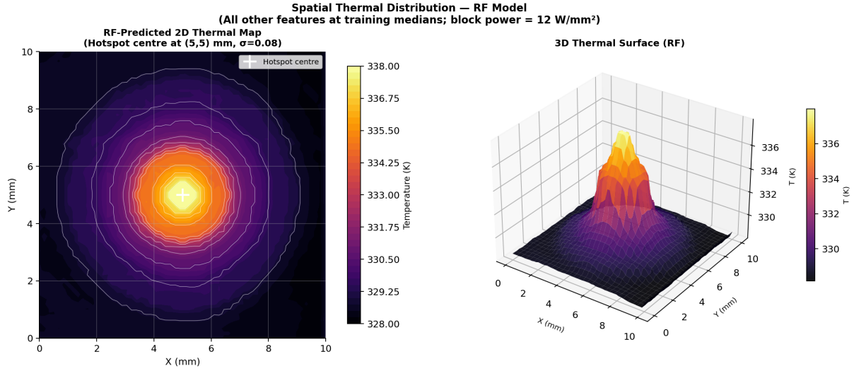
Figure 8: Left: 2D thermal map predicted by the RF model, with the hotspot centre fixed at (5 mm, 5 mm) and \sigma = 0.08 (a sharp hotspot). Contour lines show isotherms; the white cross marks the hotspot centre. Right: the same prediction as a 3D surface plot, clearly showing the Gaussian peak shape. The temperature ranges from about 328 K at the edges to \sim 338 K at the hotspot centre, a 10 K spatial variation. All other features are held at their training median values.
