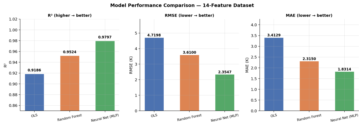
Figure 5: Side-by-side bar charts comparing R^2 , RMSE, and MAE across all model classes. The clear trend from left to right (OLS → RF → MLP) corresponds to increasing model expressiveness.
