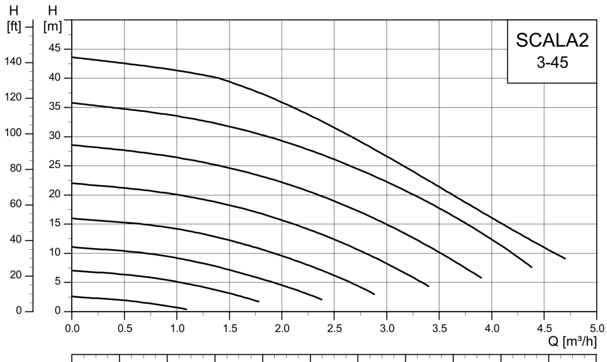
HEAD VS FLOW . 50/60 HZ
