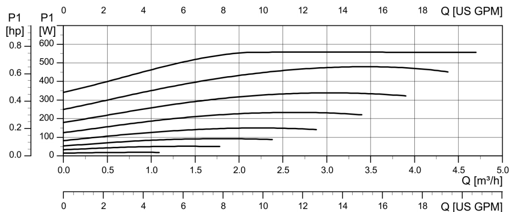
POWER INPUT P1 VS FLOW
