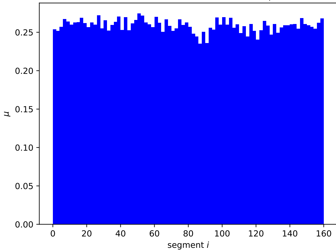
ykgE mean wildtype expression \mu_i^*
