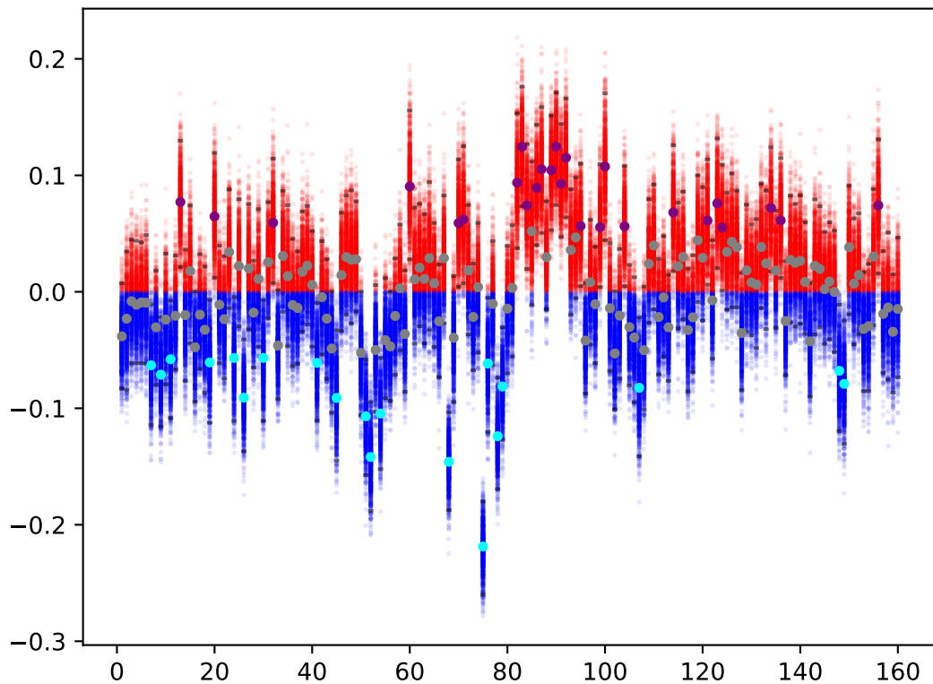
Bootstrapped \xi_i[01, 10]
