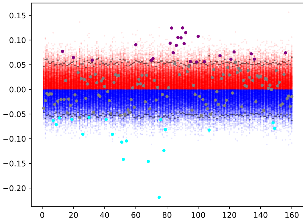
Null model \xi_i[01, 10]
