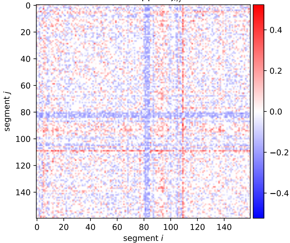
Boostrapped \xi_{i,j}
