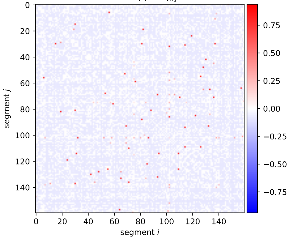
Boostrapped \xi_{i,j}
