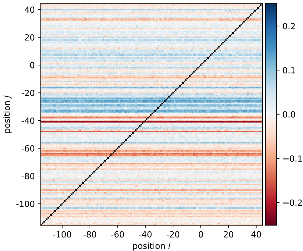
\xi[i, j] for right mutation across 2 segments
