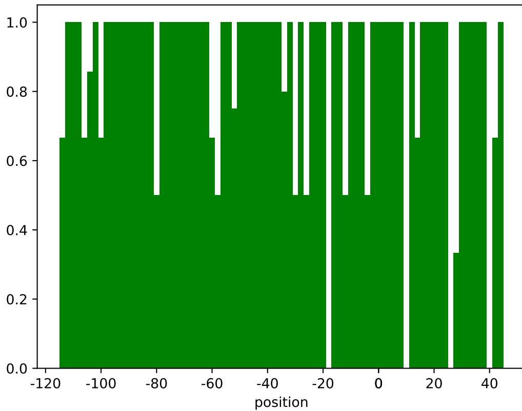
\mu_i[01] (doublets)
