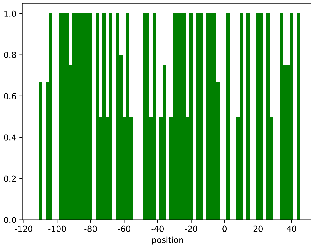
\mu_i[10] (doublets)
