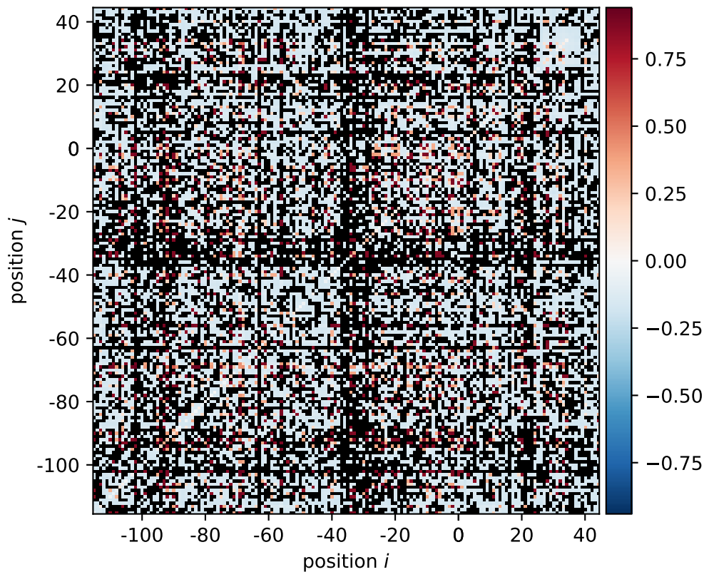
\xi[i, j] for 2 mutations across 2 segments
