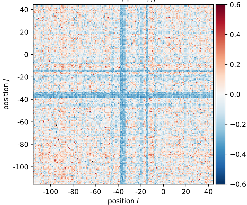
Boostrapped \xi_{i,j}
