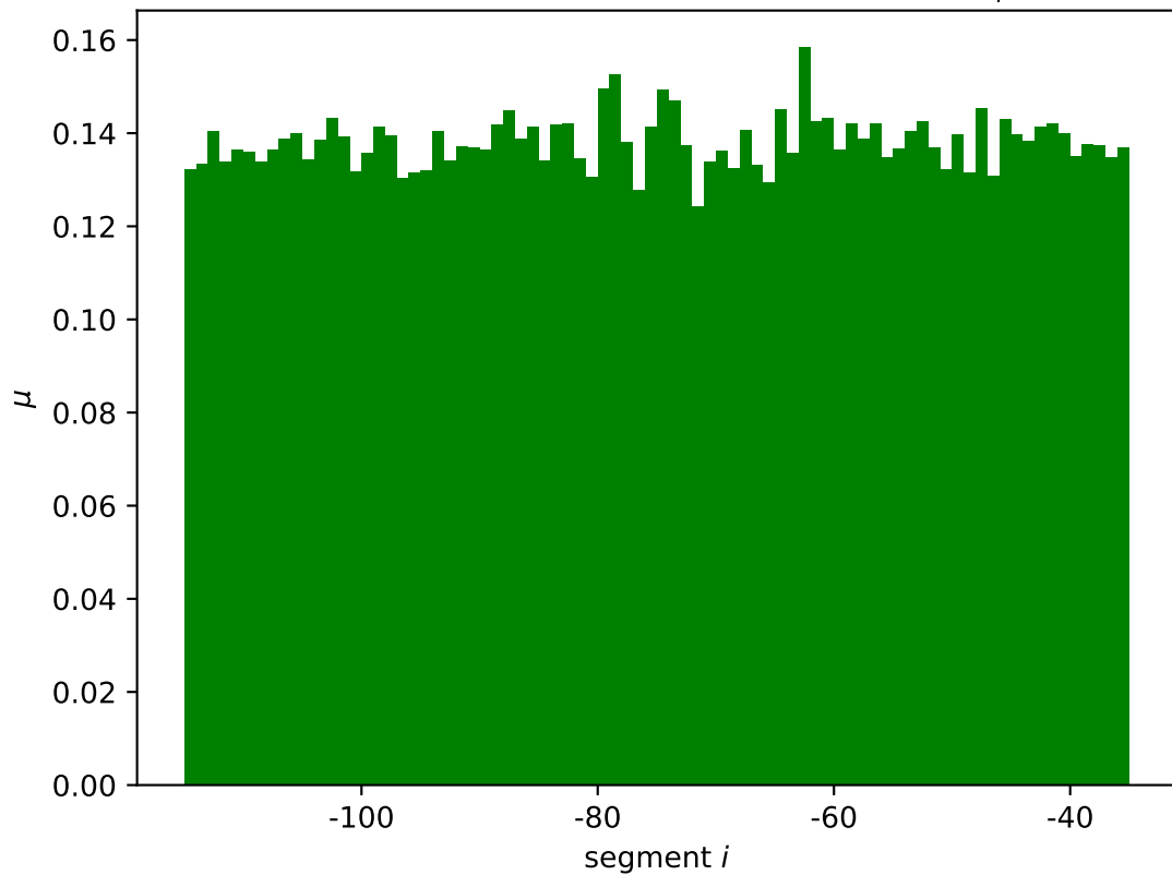
WaaA-coaD mean wildtype expression \mu_i^*
