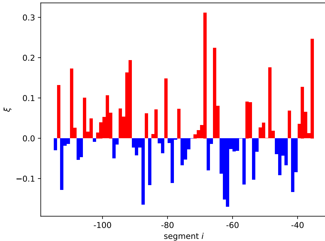
WaaA-coaD expression shift \xi_i[11]
