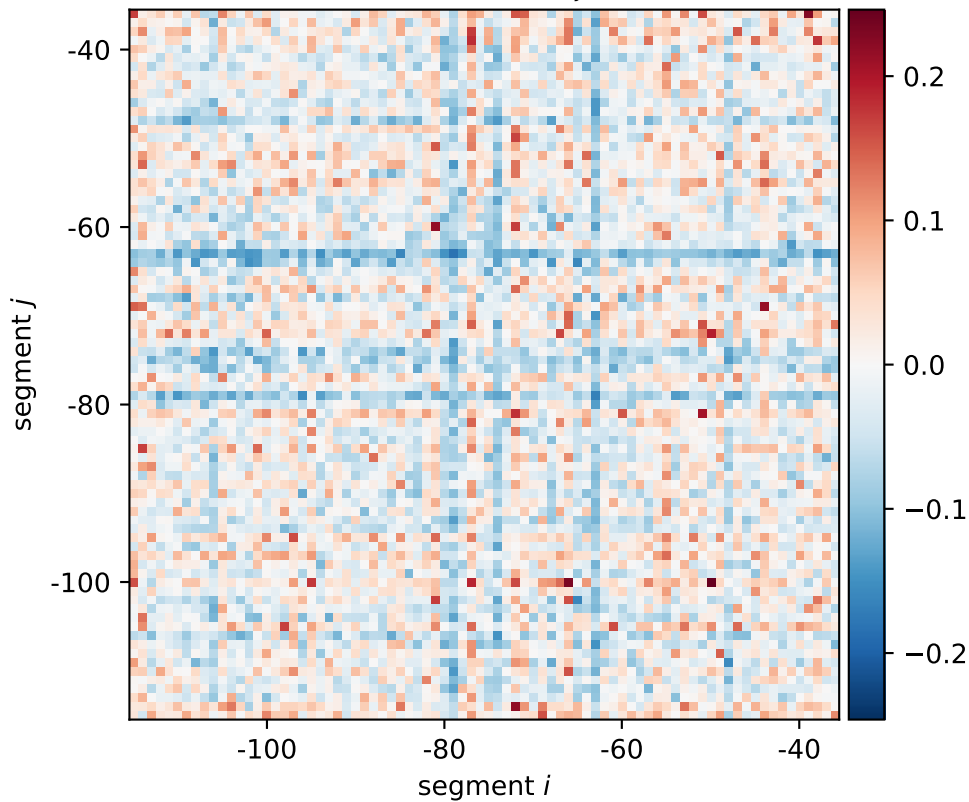
WaaA-coaD expression shift \xi_{i,j}[0101, 0110, 1010]
