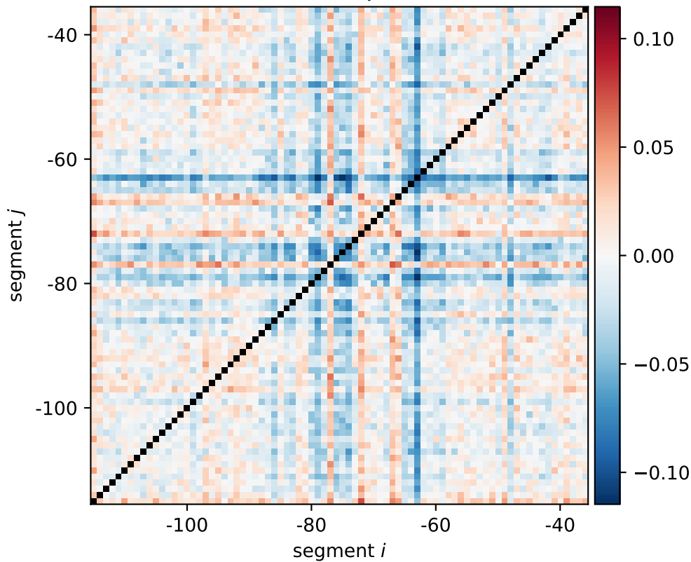
WaaA-coaD expression shift \xi_{i,j}[0001, 0010, 0100, 1000]
