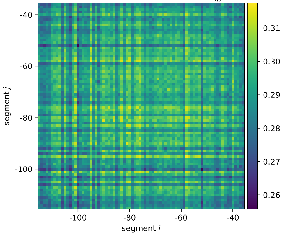
adiY mean wildtype expression \mu_{i,j}^*
