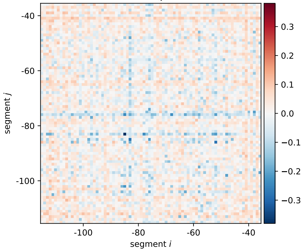
adiY expression shift \xi_{i,j}[0101, 0110, 1010]
