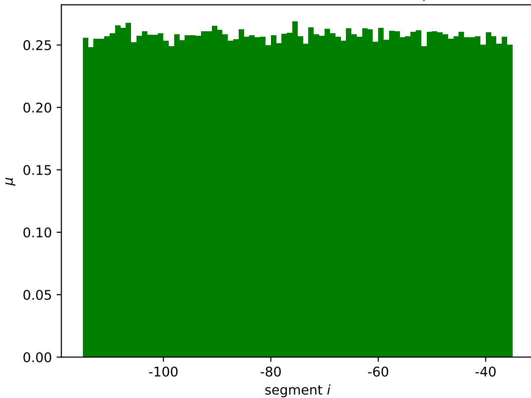
adiY mean wildtype expression \mu_i^*
