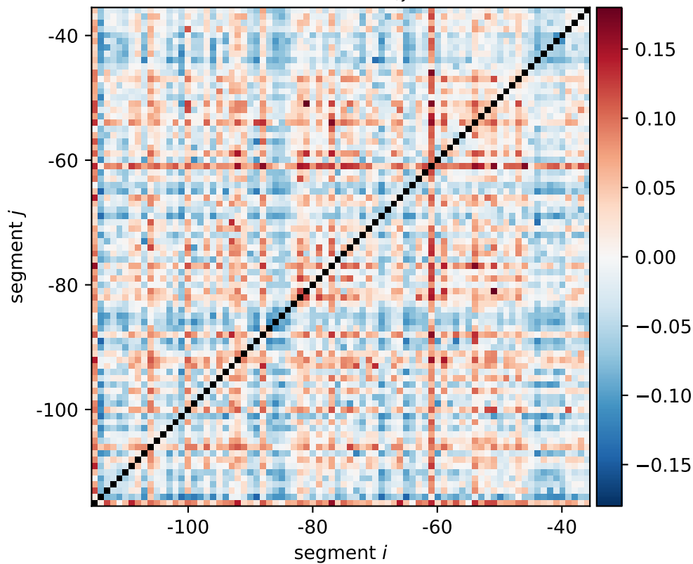
aphA expression shift \xi_{i,j}[\text{0011}, \text{1100}]
