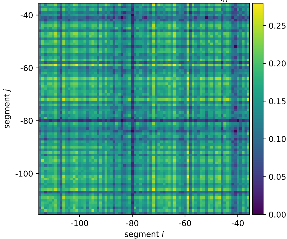
aphA mean wildtype expression \mu_{i,j}^*
