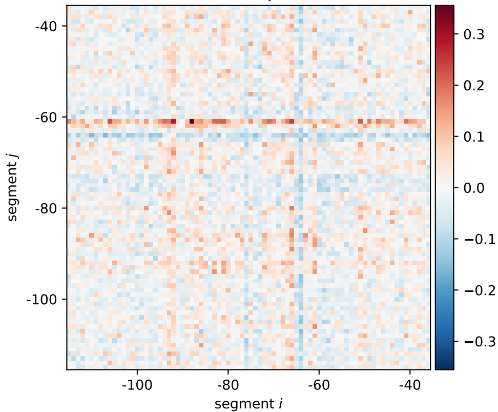
aphA expression shift \xi_{i,j}[0101, 0110, 1010]
