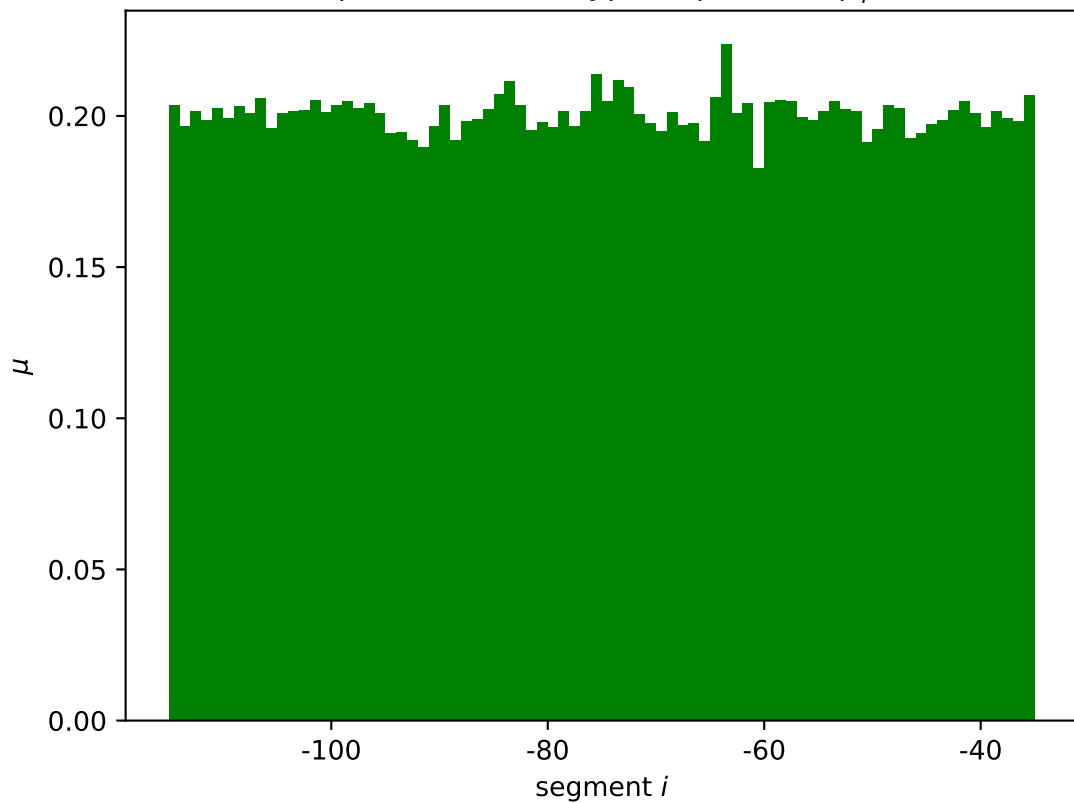
aphA mean wildtype expression \mu_i^*
