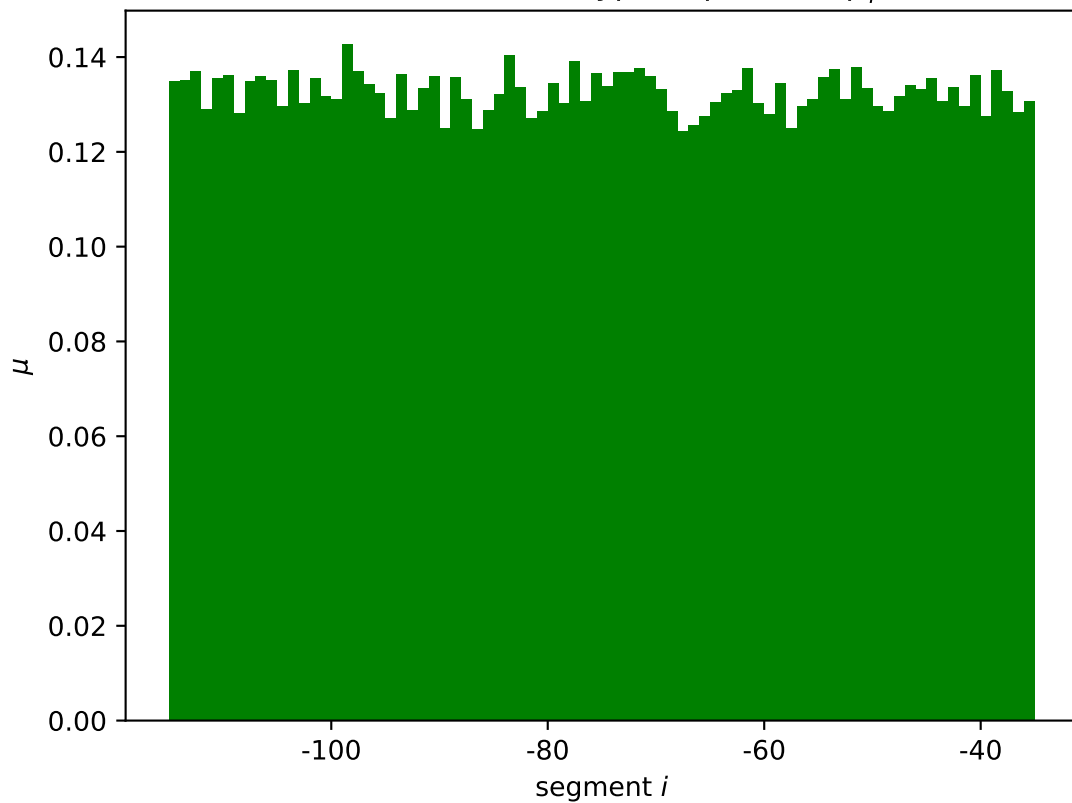
araAB mean wildtype expression \mu_i^*
