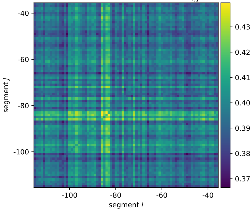
araC mean wildtype expression \mu_{i,j}^*
