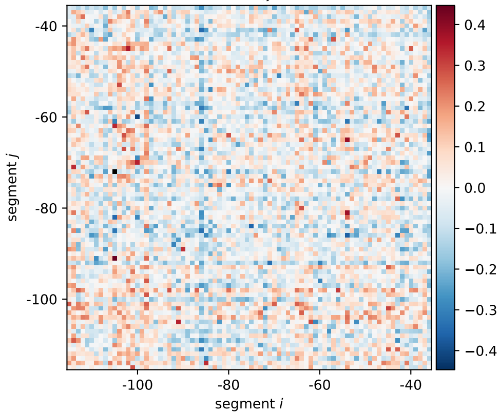
araC expression shift \xi_{i,j}[\text{0101}, \text{0110}, \text{1010}]
