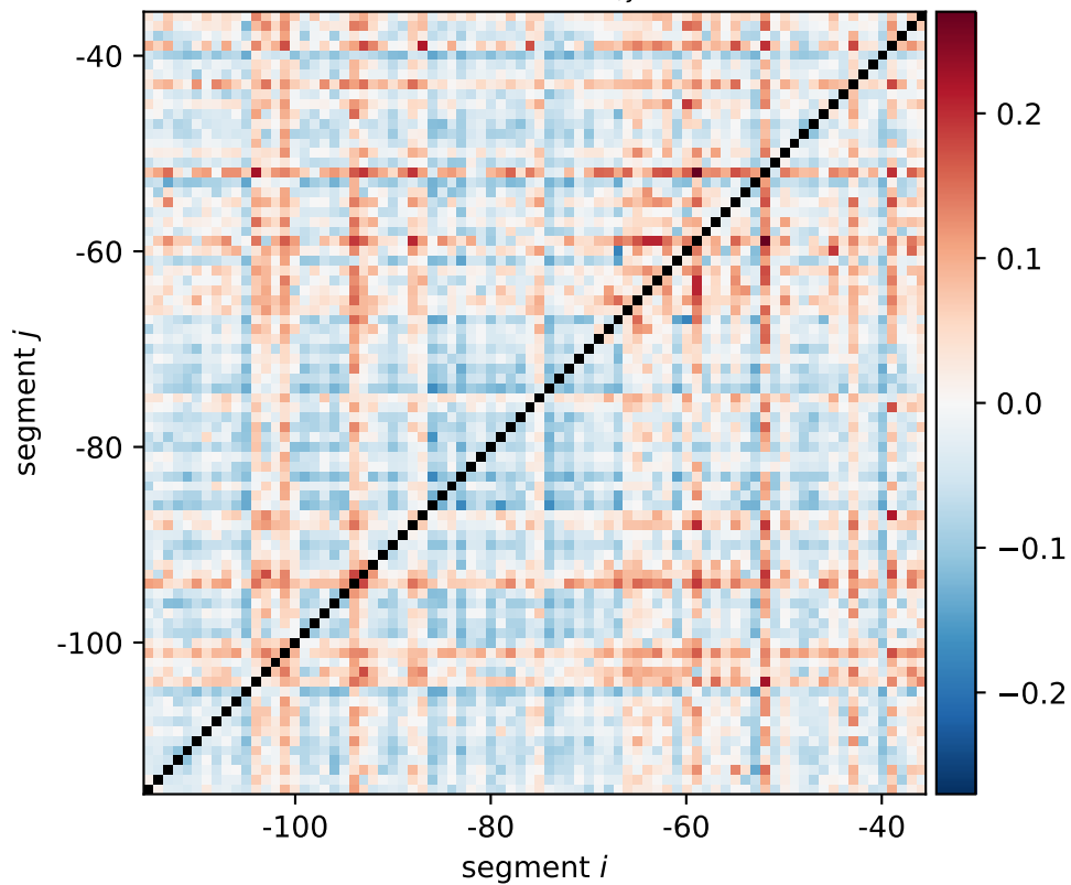
araC expression shift \xi_{i,j}[0011, 1100]
