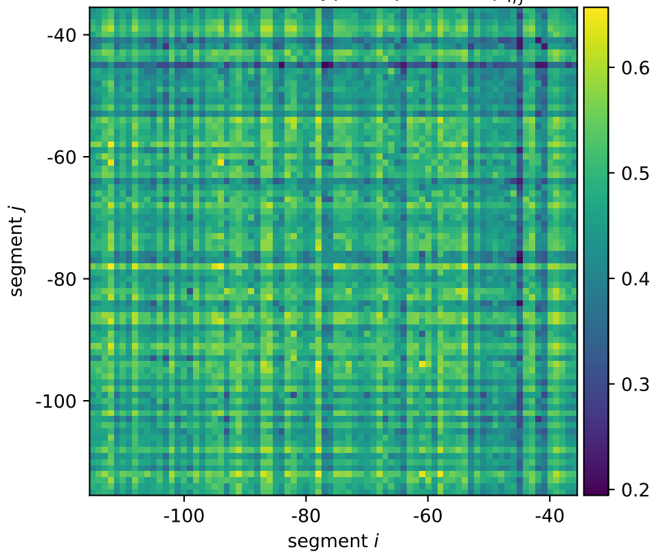
arcA mean wildtype expression \mu_{i,j}^*
