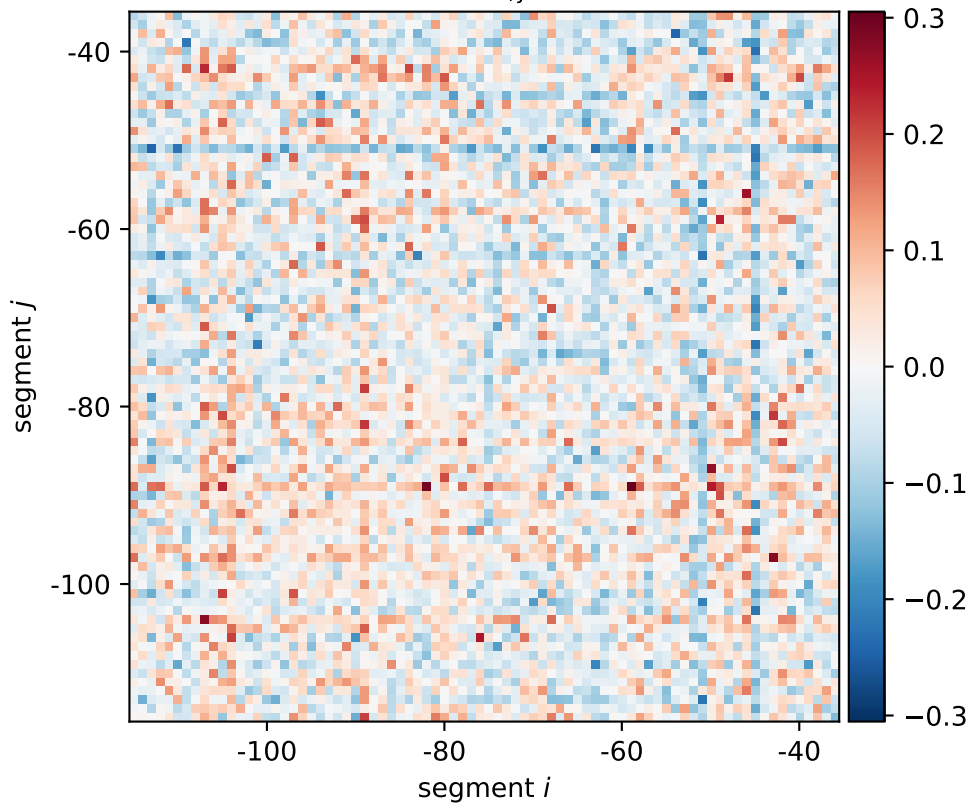
arcB expression shift \xi_{i,j}[0101, 0110, 1010]
