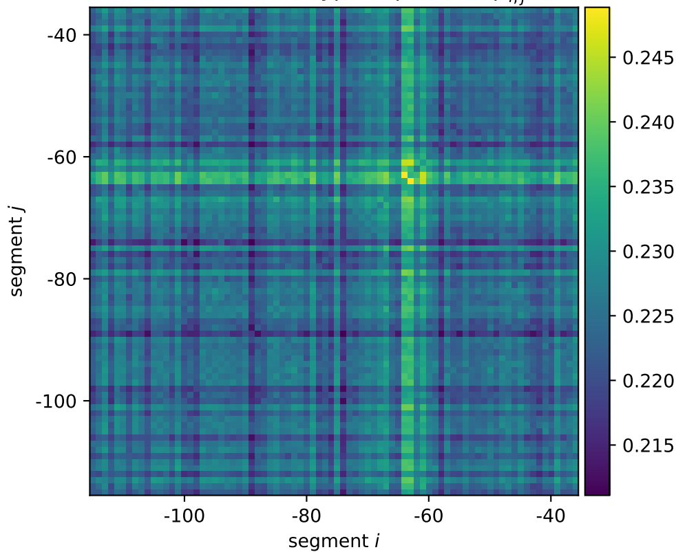
arcB mean wildtype expression \mu_{i,j}^*
