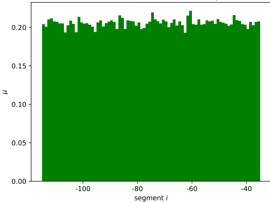
asnA mean wildtype expression \mu_i^*
