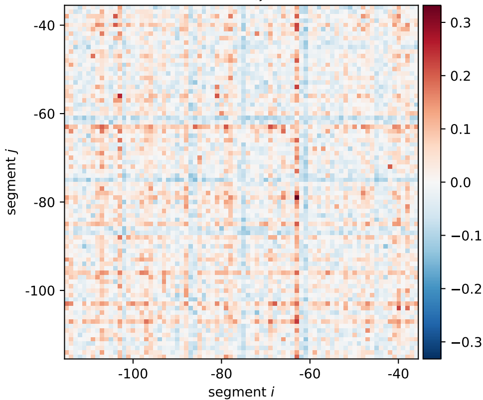
asnA expression shift \xi_{i,j}[0101, 0110, 1010]
