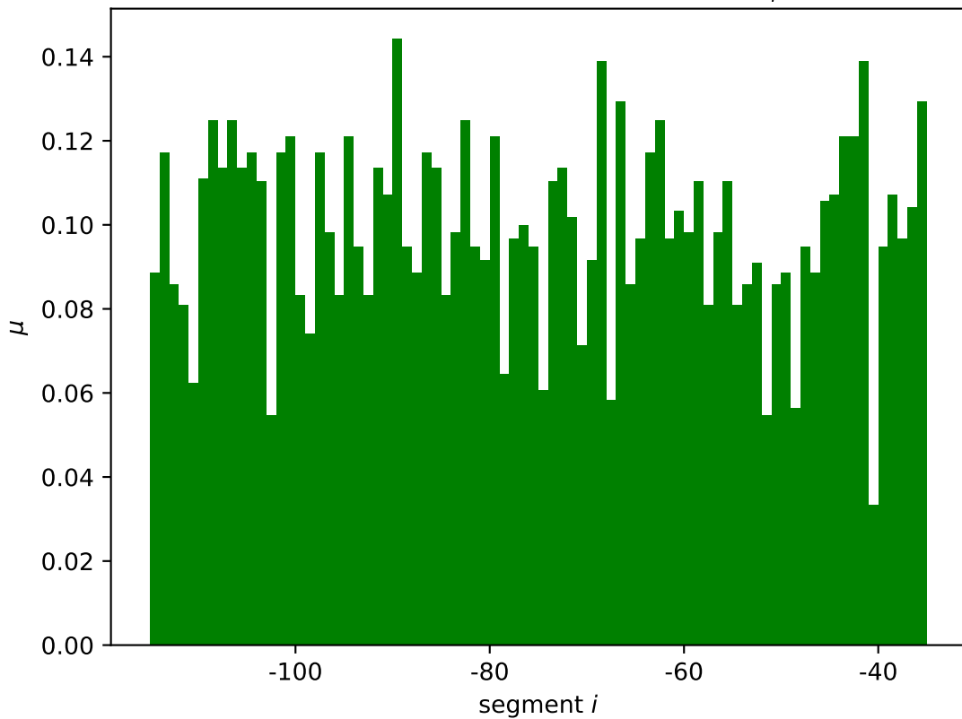
bdcR mean wildtype expression \mu_i^*
