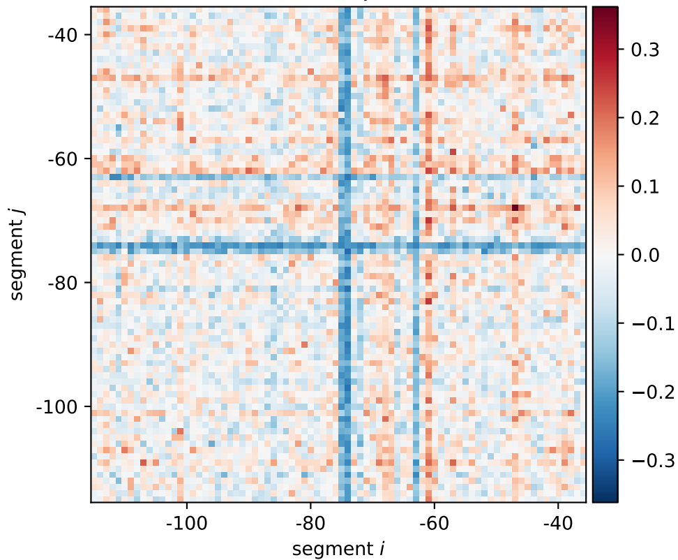
bdcR expression shift \xi_{i,j}[0101, 0110, 1010]
