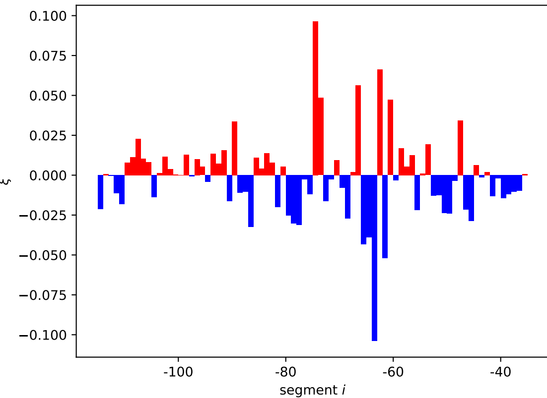
coaA expression shift \xi_i[01, 10]
