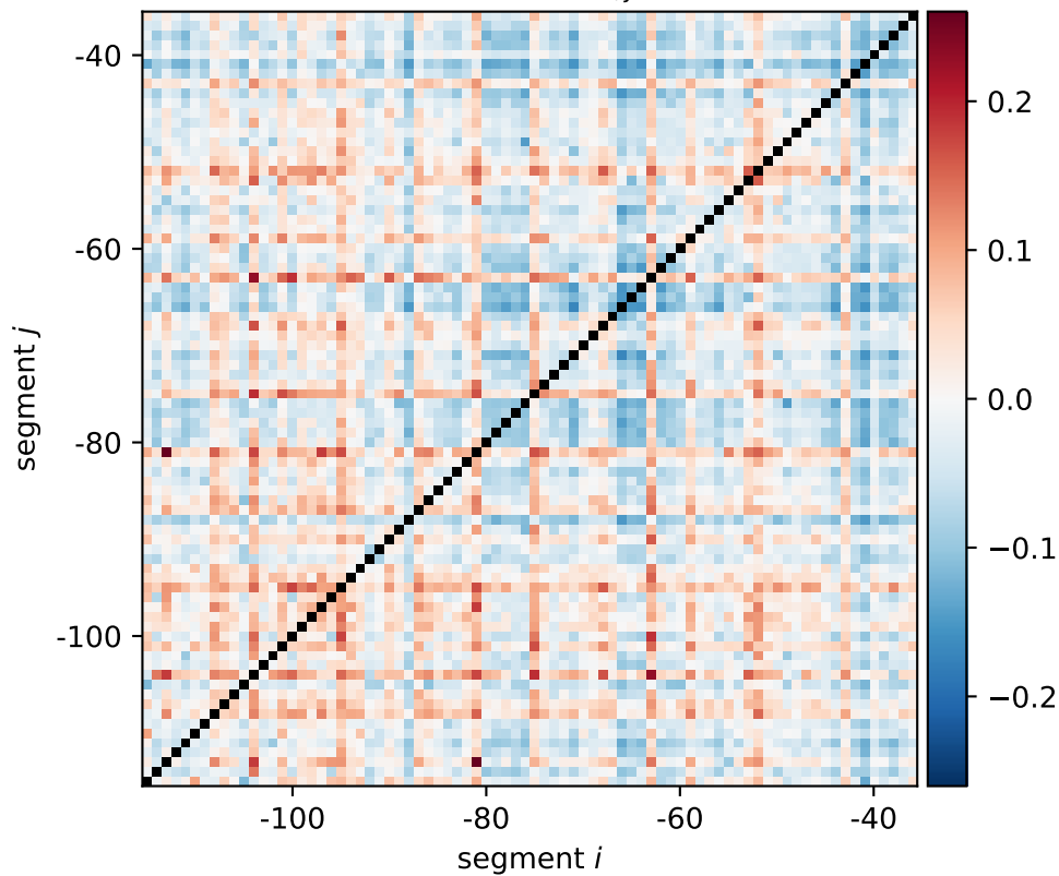
coaA expression shift \xi_{i,j}[0011, 1100]
