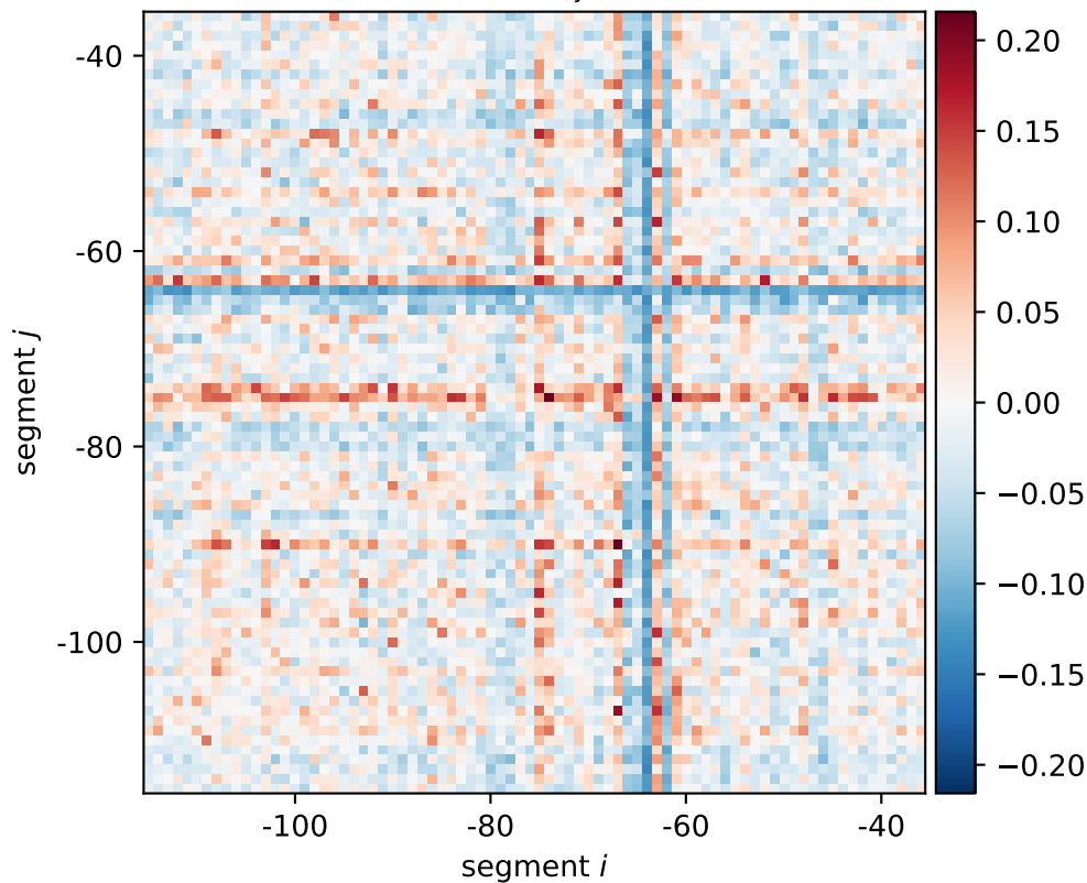
coaA expression shift \xi_{i,j}[0101, 0110, 1010]
