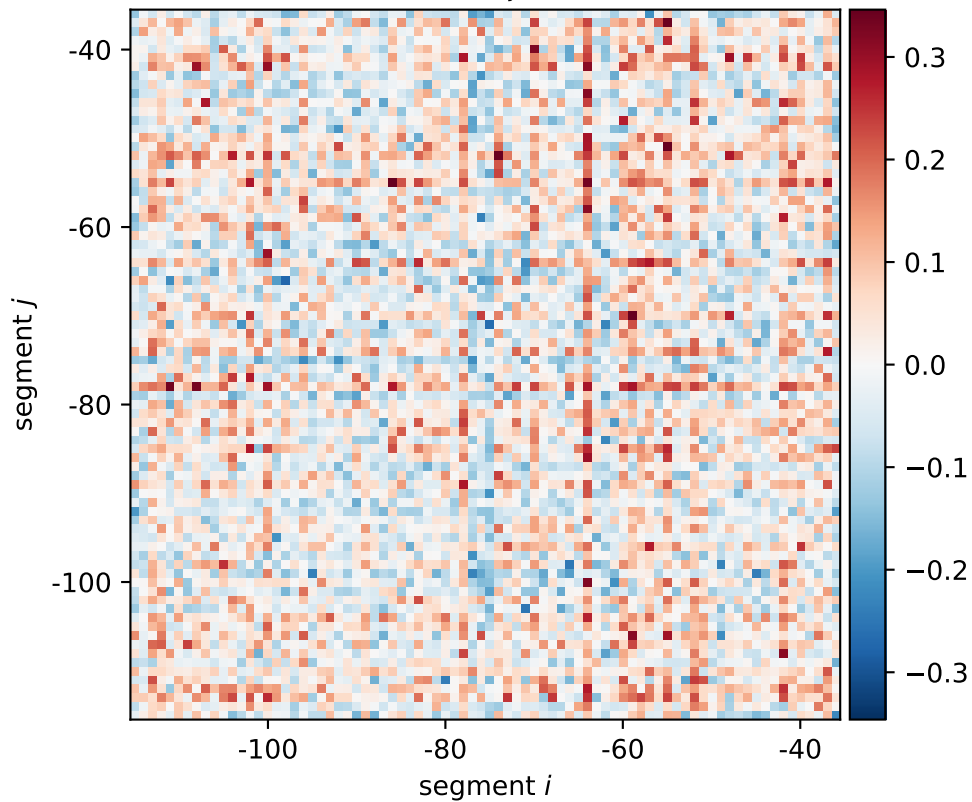
cra expression shift \xi_{i,j}[0101, 0110, 1010]
